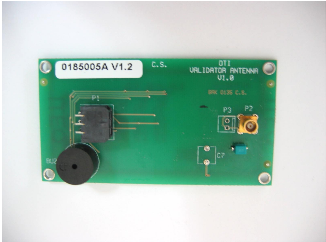
Photograph No.6 Contactless card reader Antenna PCB front view
