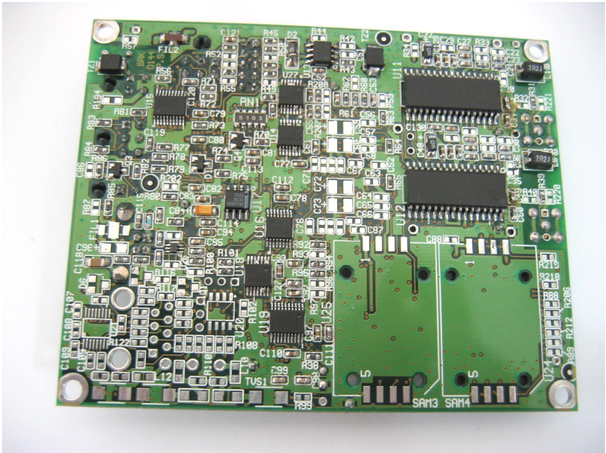
Photograph No.4 Contactless card reader PCB second side view
