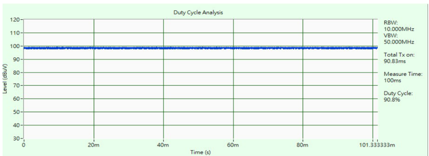
Time-domain plot for Bluetooth transmission signal
