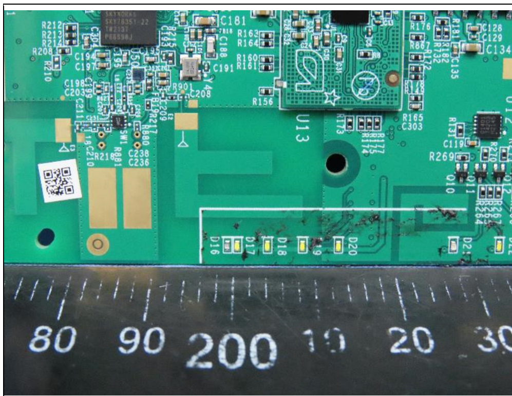
Antenna (SRD Ant E2)
