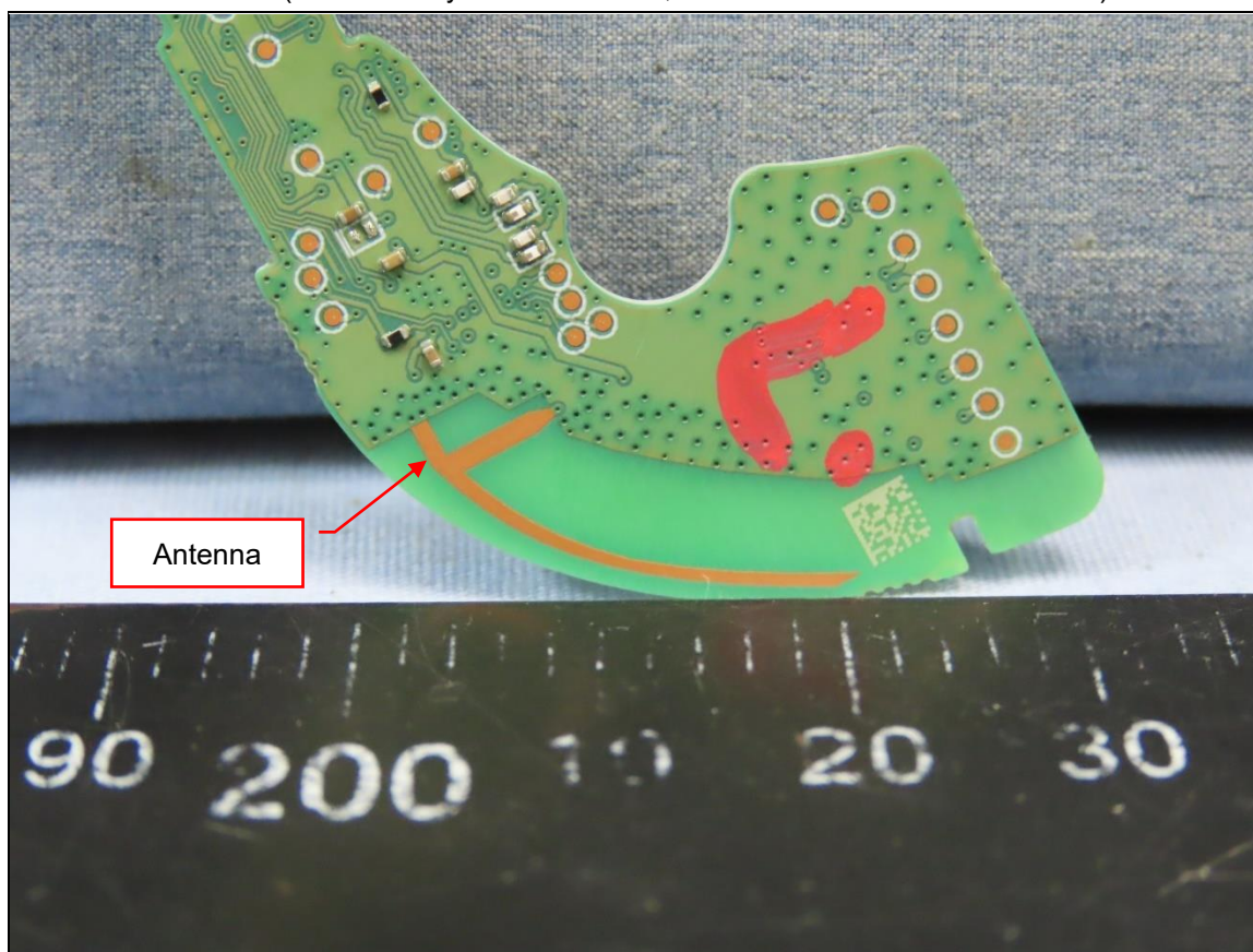
Antenna (Brand: Merry Electronics Co., Ltd. / Model: 52TX5892000LZ-M)
