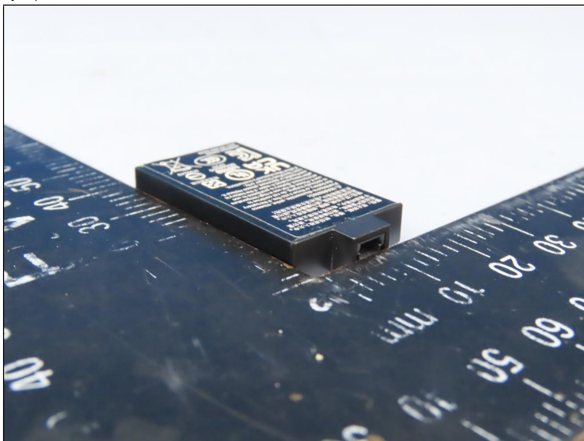
Battery 2 (Brand: VIETNAM EXQUISITE POWER TECHNOLOGY COMPANY LIMITED / Model: 521630-A)
