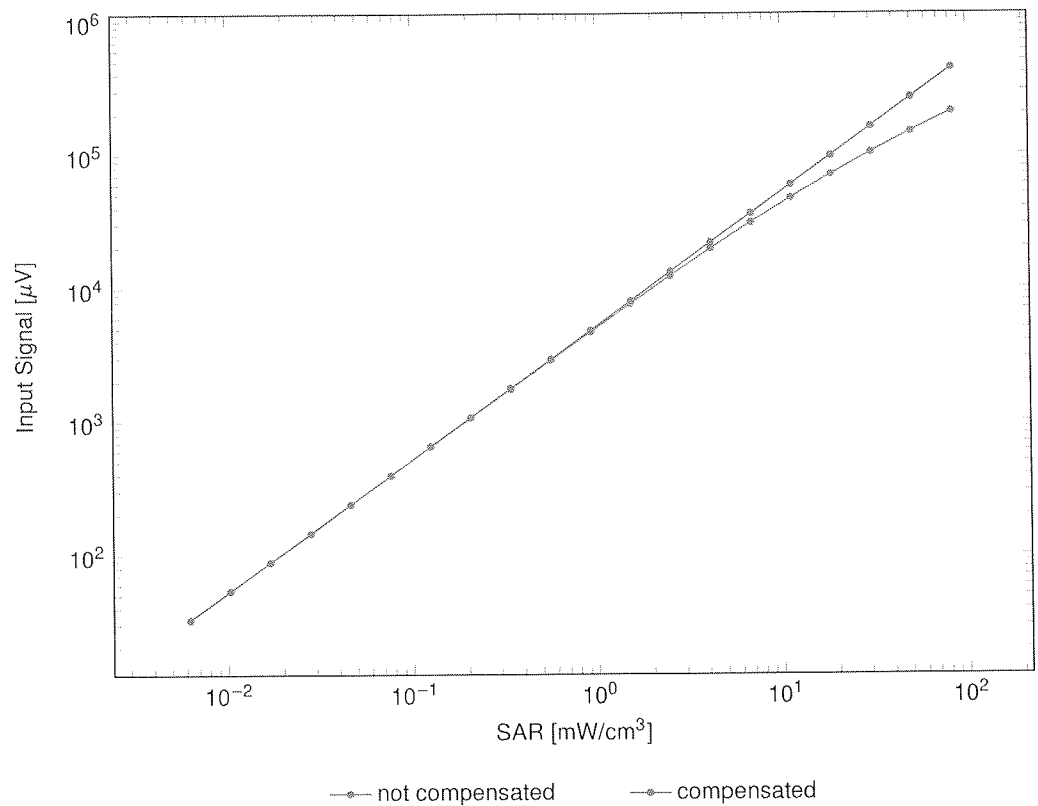
Dynamic Range f(\text{SAR}_{\text{HSL}}) (TEM cell, f_{\text{eval}} = 1900 \text{ MHz} )
