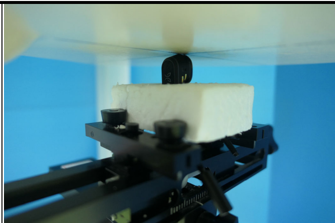
Bottom Side of Left Ear EUT Tested at 0 mm
