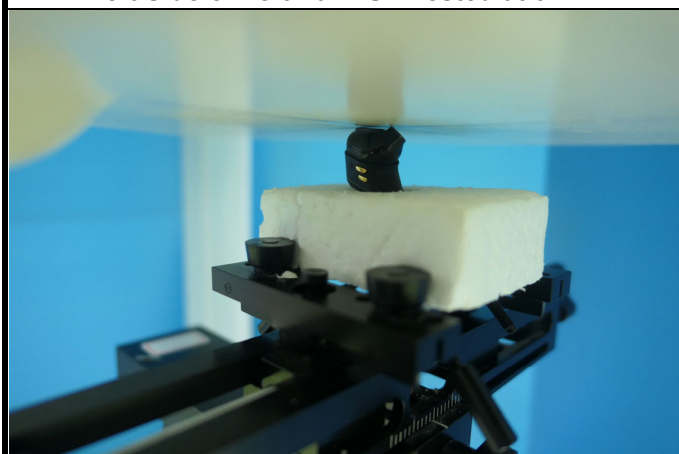
Rear Face of Left Ear EUT Tested at 0 mm
