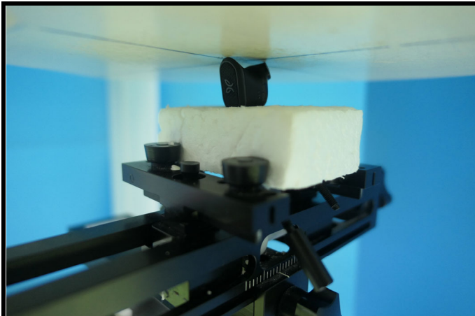
Top Side of Left Ear EUT Tested at 0 mm
