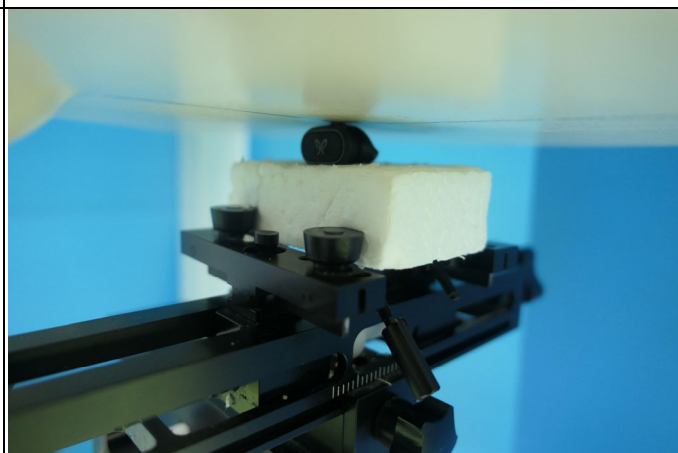
Right Side of Left Ear EUT Tested at 0 mm
