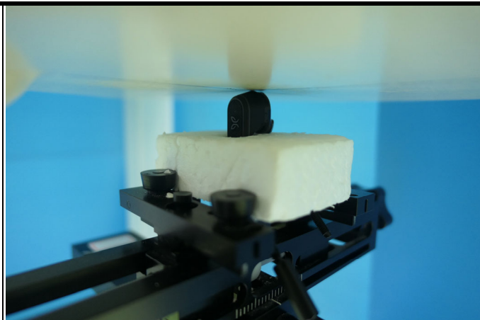
Bottom Side of Right Ear EUT Tested at 0 mm
