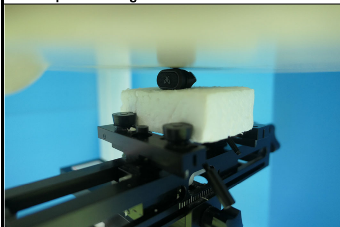
Left Side of Right Ear EUT Tested at 0 mm
