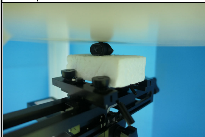
Left Side of Left Ear EUT Tested at 0 mm
