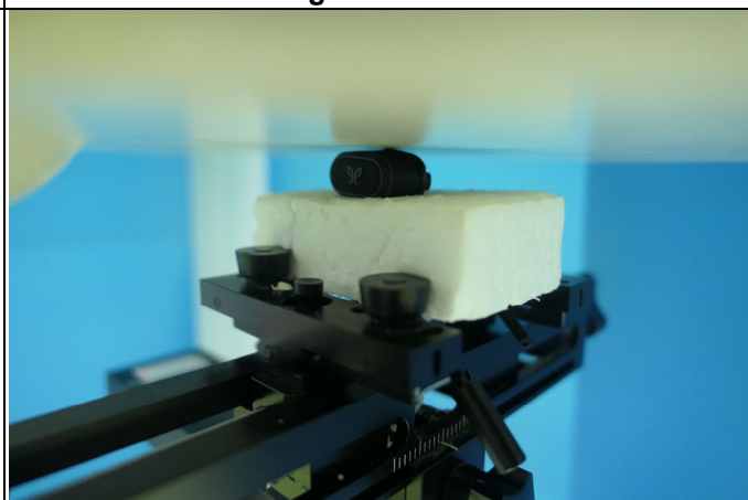
Right Side of Right Ear EUT Tested at 0 mm
