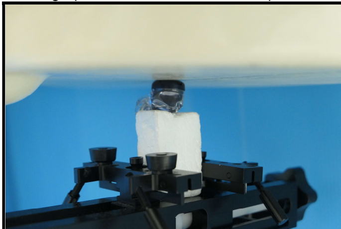
Front Face of Earphone Tested at 0 mm
