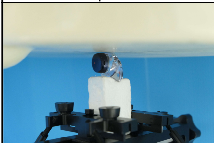
Left Side of Earphone Tested at 0 mm
