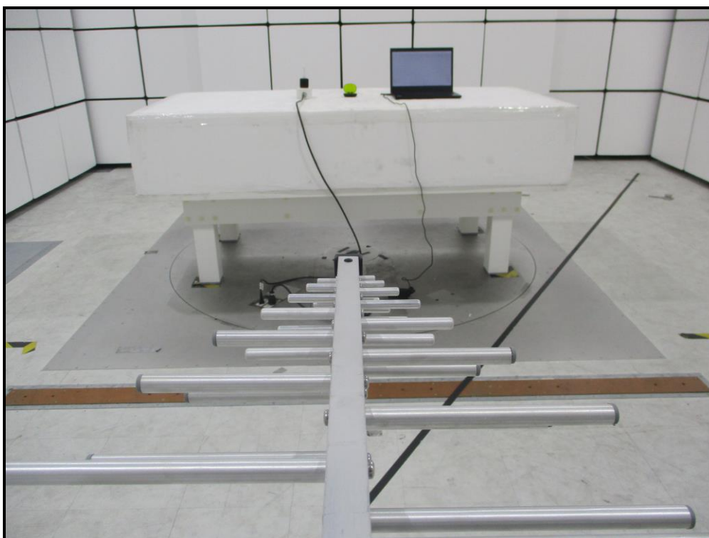
Unwanted Emissions above 1 GHz
