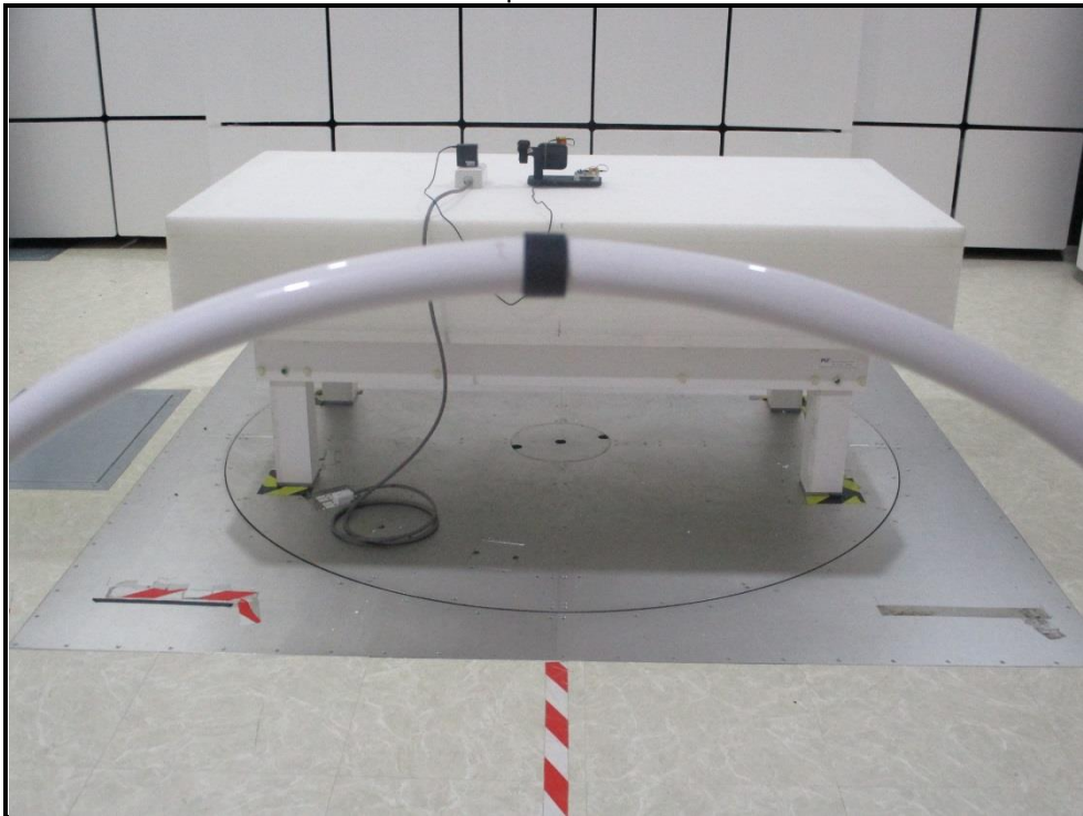
Loop Antenna
