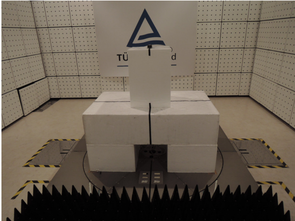
Photograph 4: Set-up for Spurious Emissions (IC)
