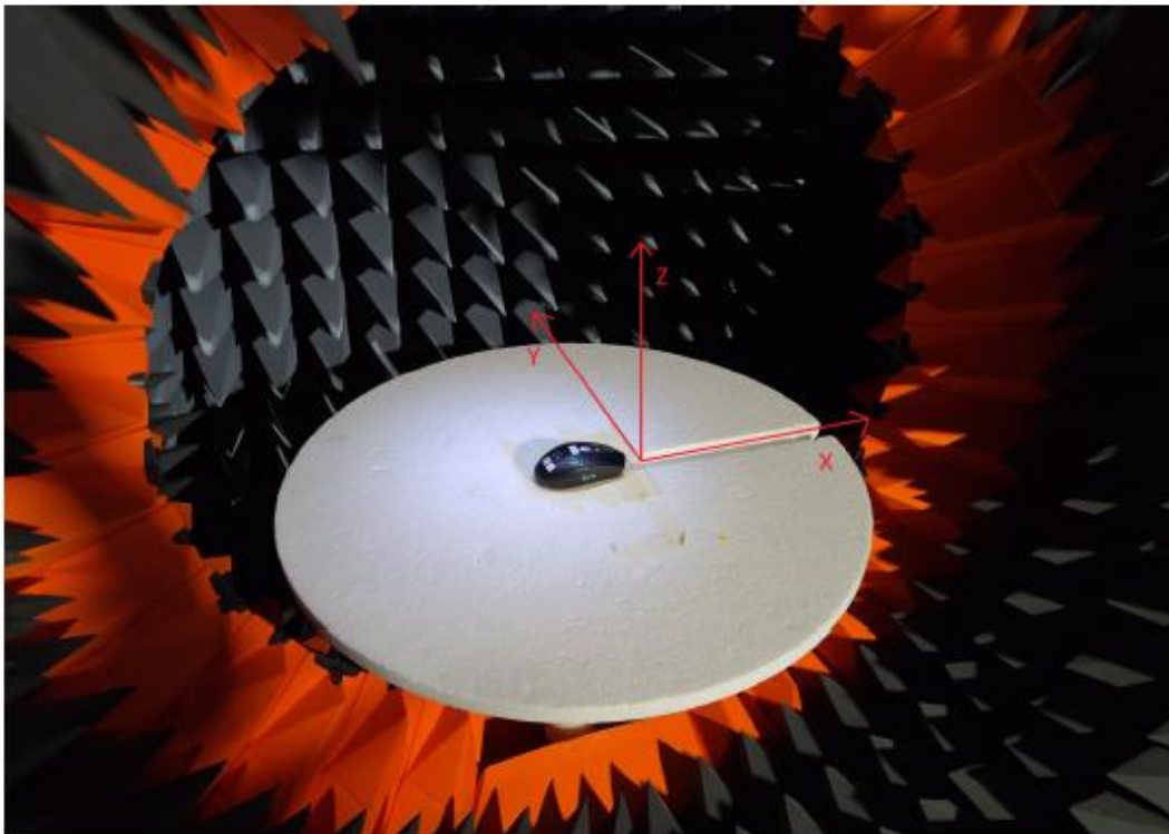
4.5 Test Setup photos
