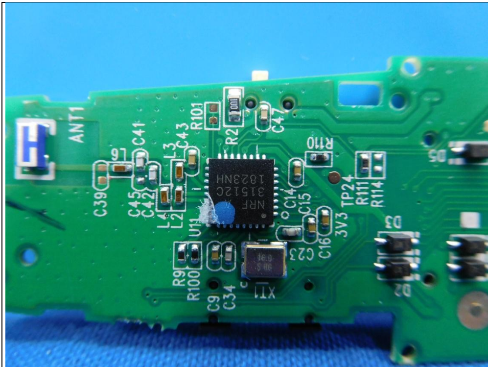
Ceramic Chip Antenna
