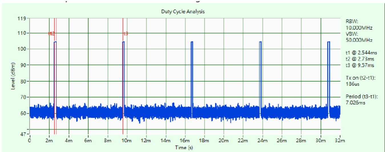
Time-domain plot for Bluetooth transmission signal
