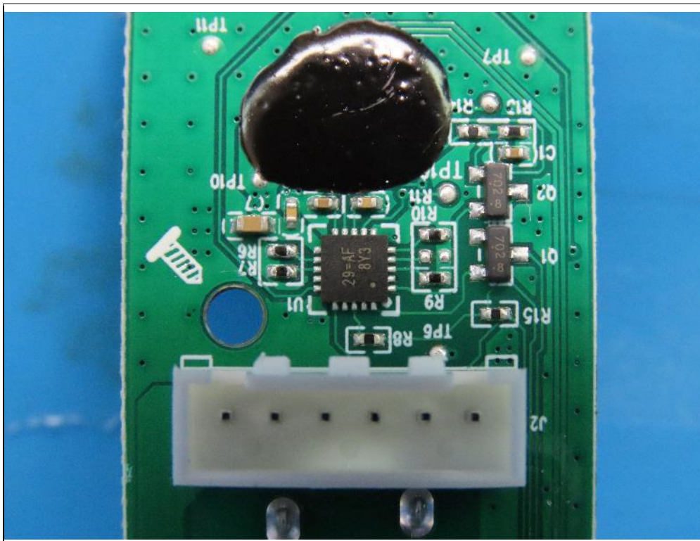
Difference (Change to PD circuit)
