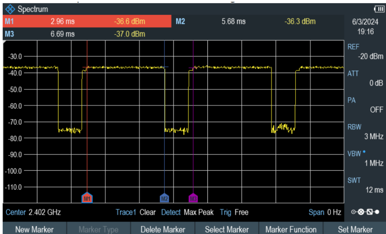
Time-domain plot for Bluetooth transmission signal
