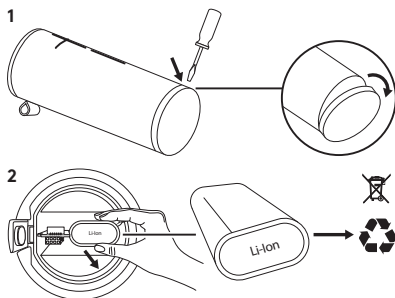
Battery Removal for Recycling
