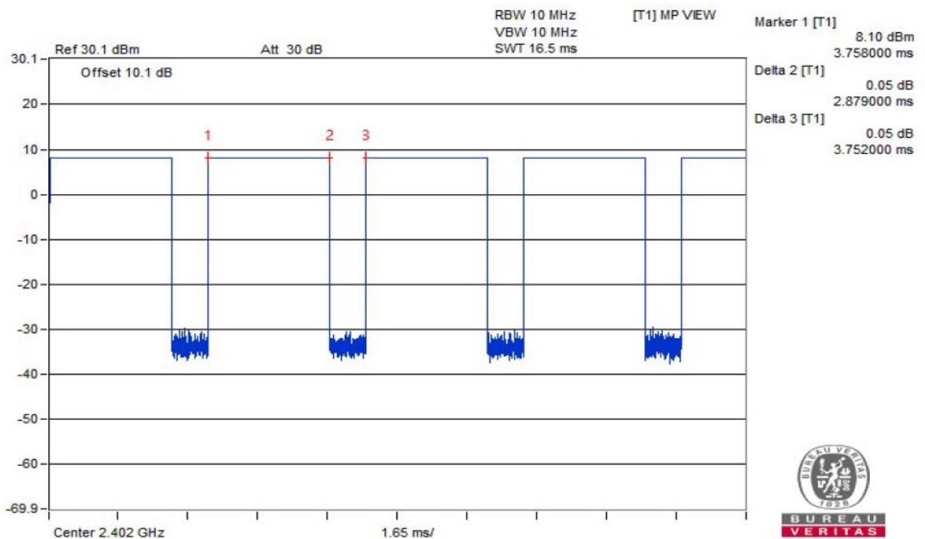
Time-domain plot for Bluetooth transmission signal
