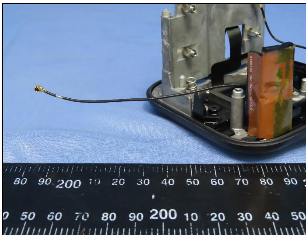
Antenna 1
