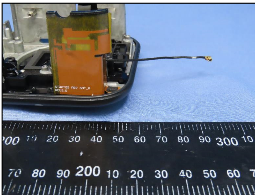
Antenna 0
