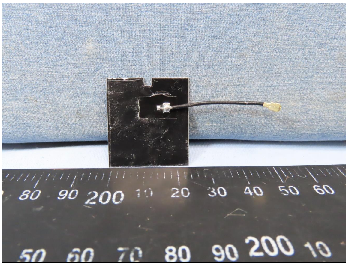
Antenna 2 (WiFi 2)
