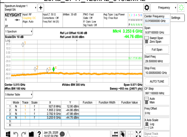
LoRa SF11 125kHz 927.6MHz
