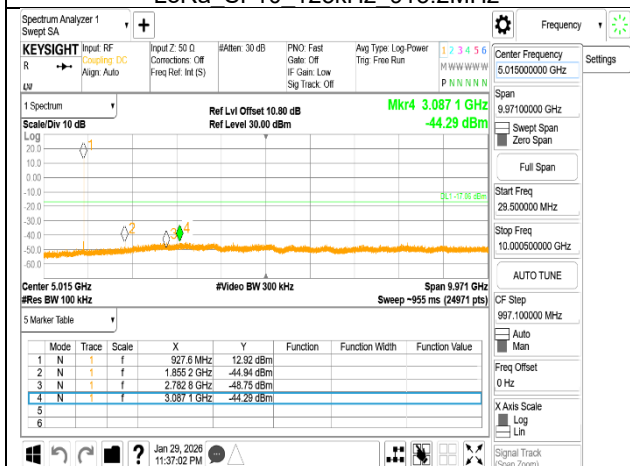
LoRa SF10 125kHz 927.6MHz
