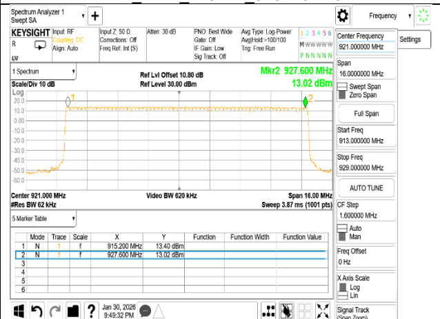
Lora_SF7_125kHz 915.2-927.6
