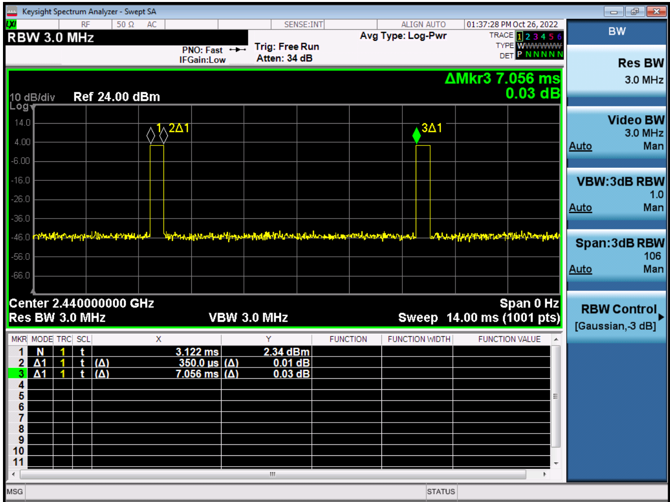
Figure 6-1 Bluetooth Transmission Plot
