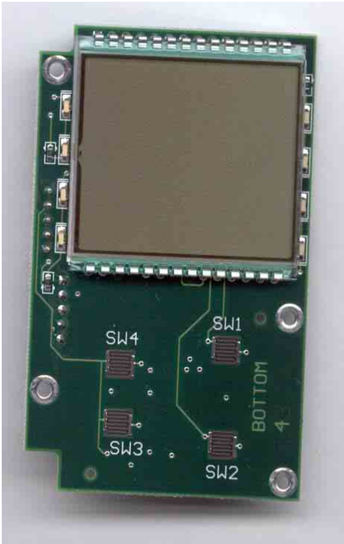
Figure 5: Display Board Front
