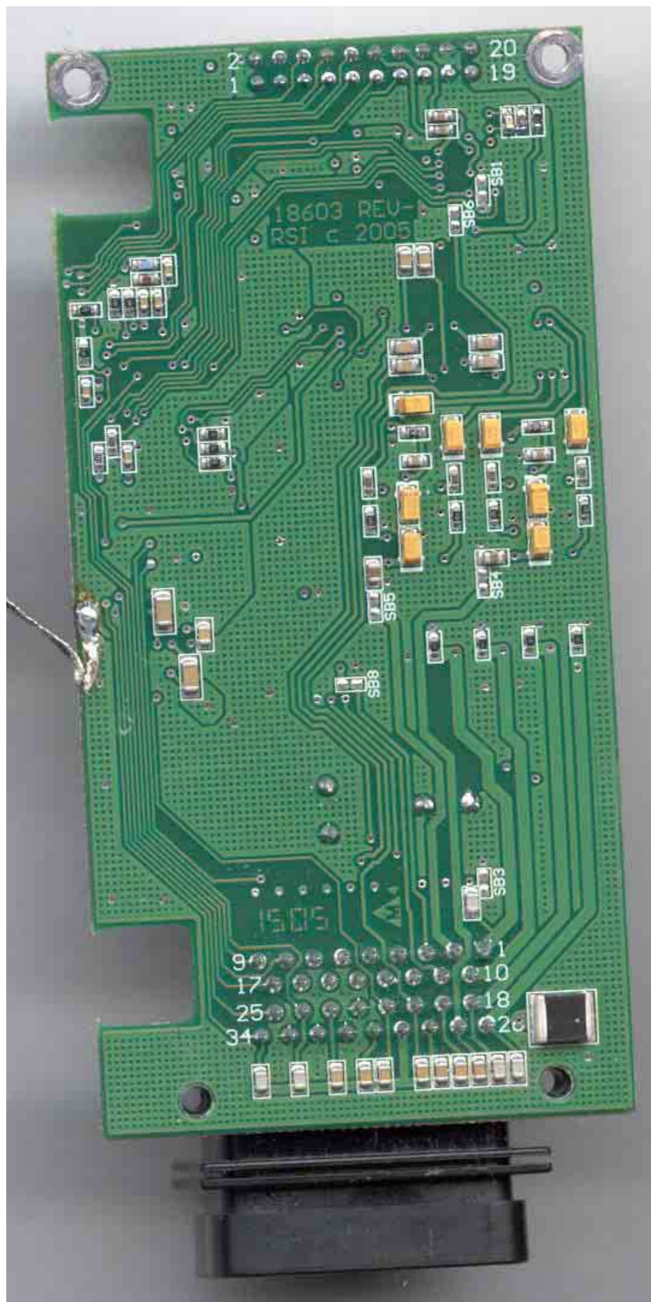
Figure 4: Audio Board Back
