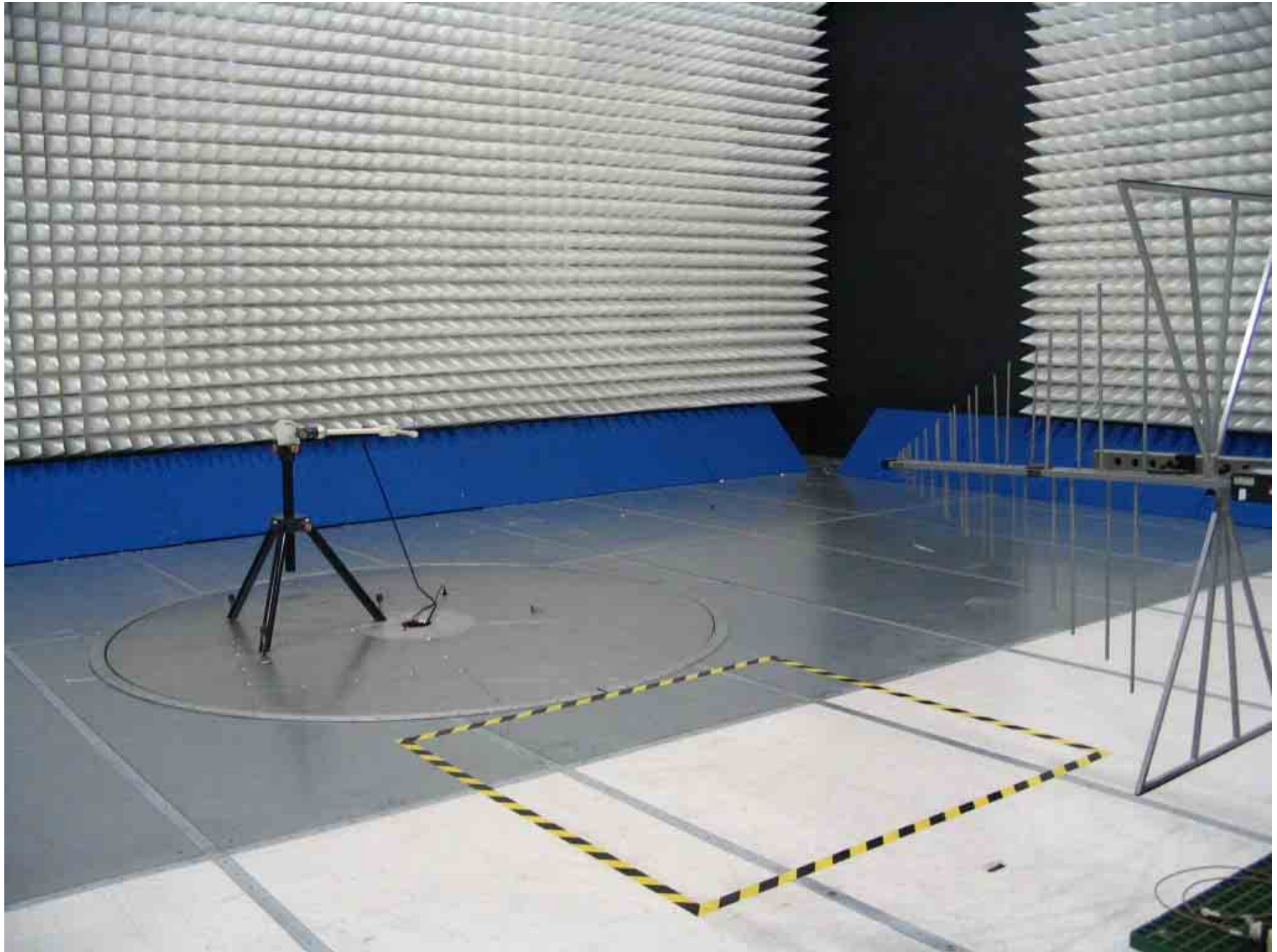
Figure 4: Substitution Measurements
