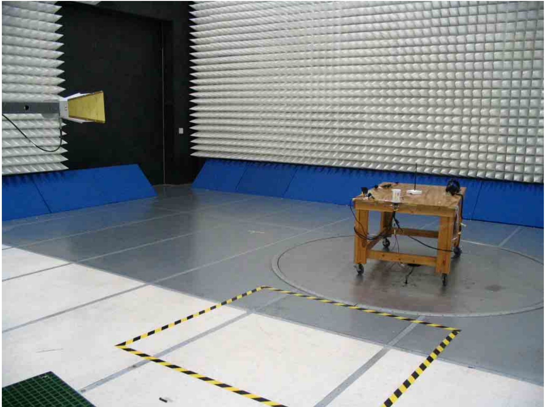
Figure 3: Radiated Testing #2
