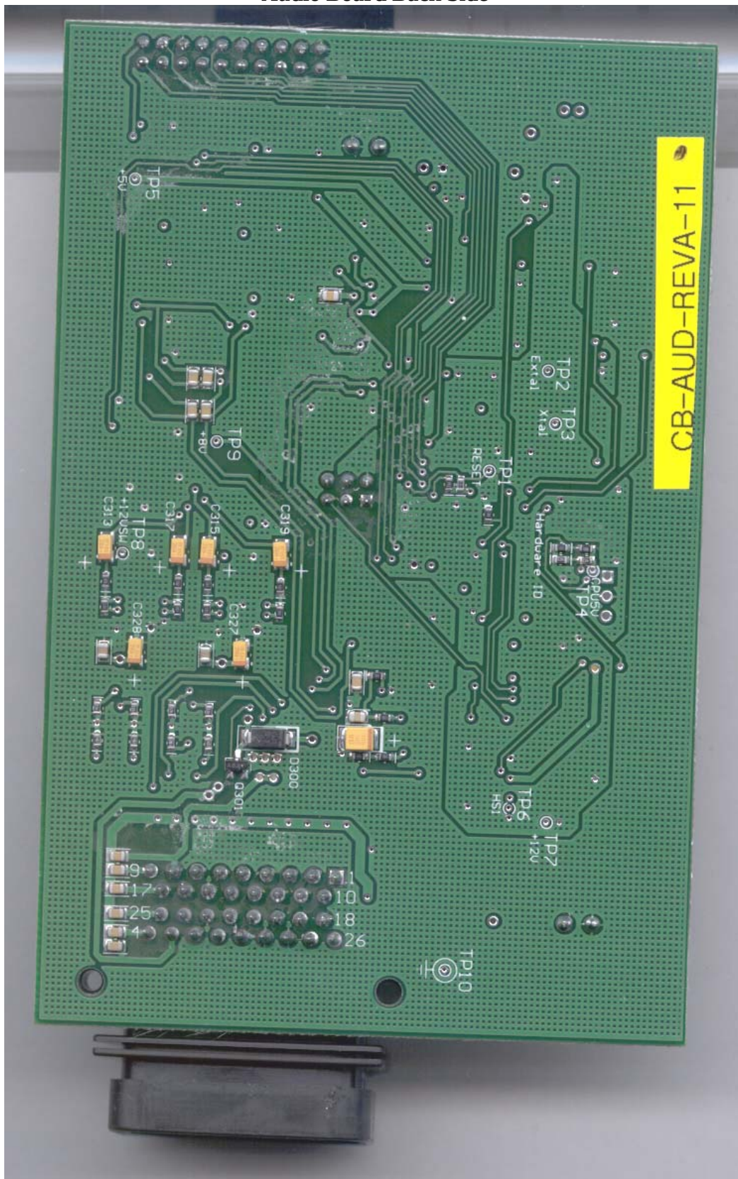
Audio Board Back Side
