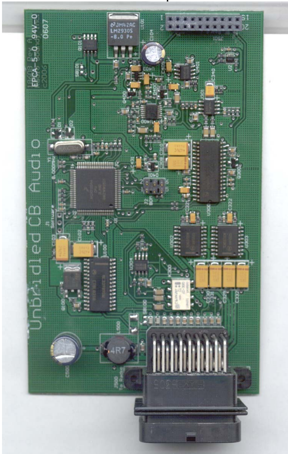
Audio Board Top Side
