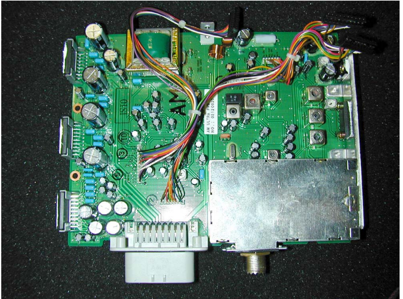
Figure 6 – Bottom PCB (Bottom)
