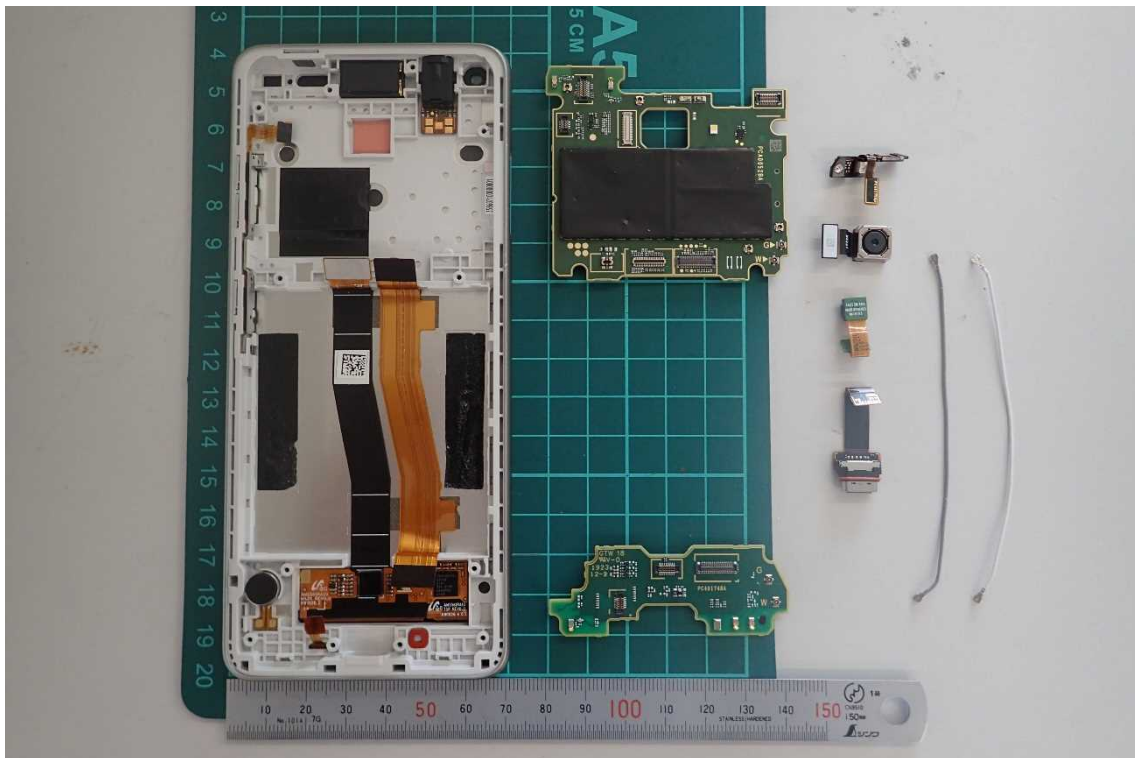
Rear cover open 4
