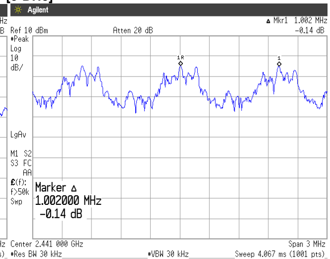
[3-DH5(AFH)]
