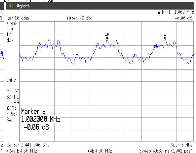
[3-DH5(AFH)]
