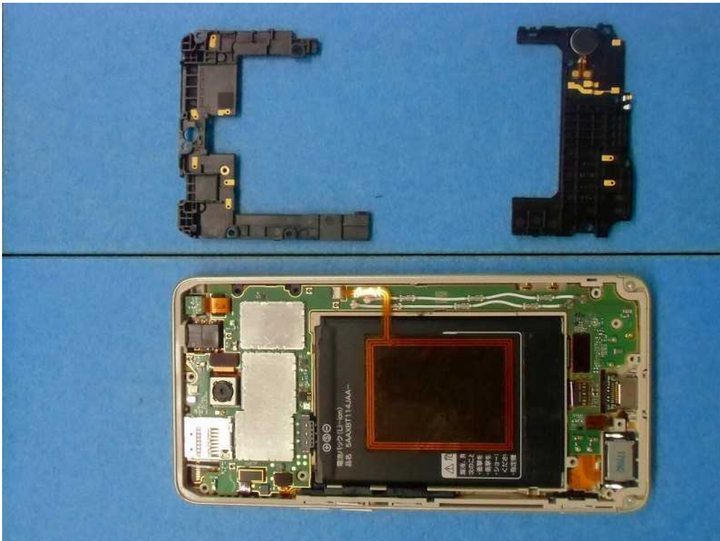
Rear cover open 1
