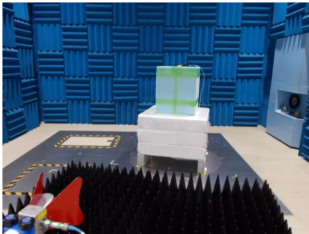
Above 1GHz
