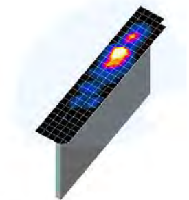
Figure 4.1 Sample SAR Area Scan
