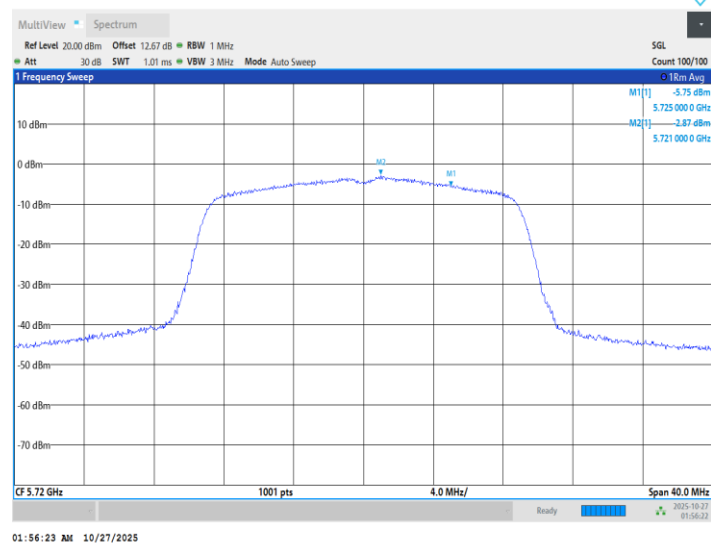
11N20SISO_Ant1_5720_UNII-3
