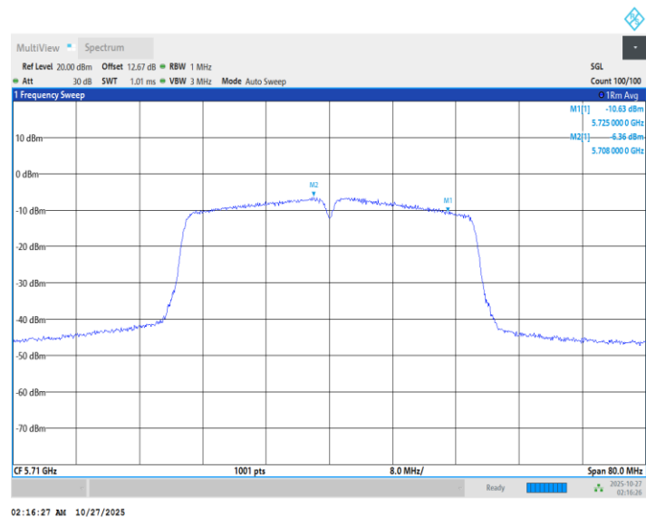
11N40SISO_Ant1_5710_UNII-3
