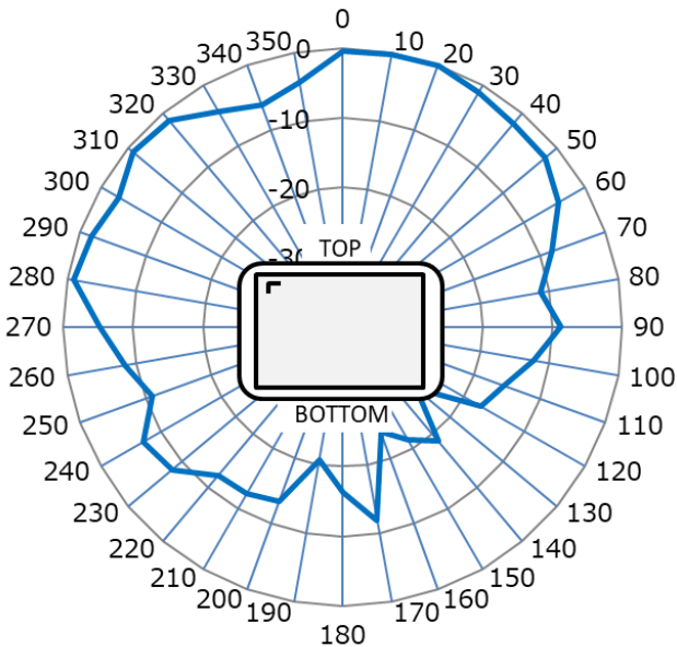
Wi-Fi BT ANT; WLAN W52_W53
