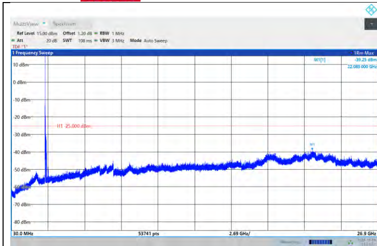
Band41-10MHz-16QAM-41540-1RB#0- Range:30~26900MHz
