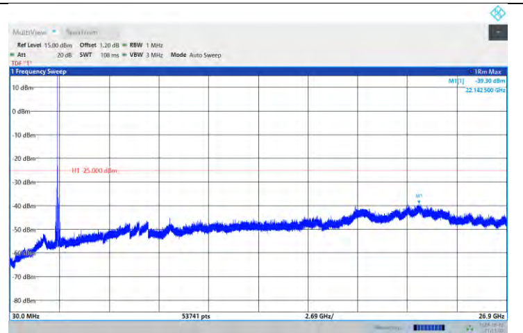
Band41-10MHz-64QAM-39700-1RB#0-Range:30~26900MHz
