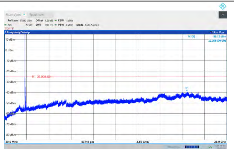
Band41-10MHz-64QAM-41540-1RB#0-Range:30~26900MHz
