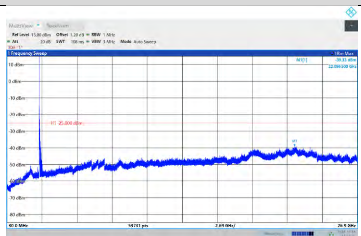
Band41-20MHz-QPSK-41490-1RB#0-Range:30~26900MHz
