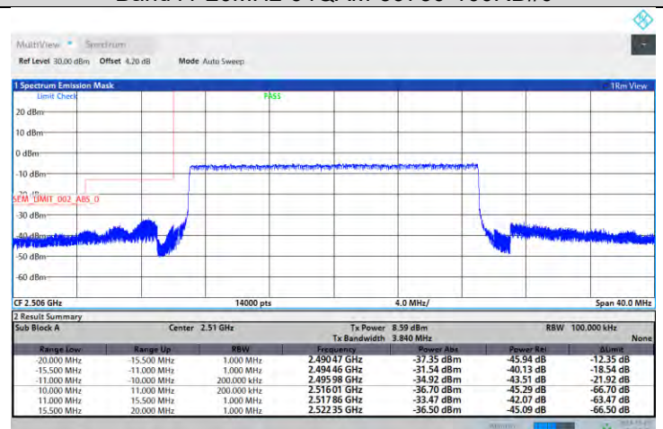
Band41-20MHz-64QAM-41490-100RB#0
