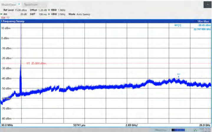
Band41-5MHz-16QAM-39675-1RB#0-Range:30~26900MHz
