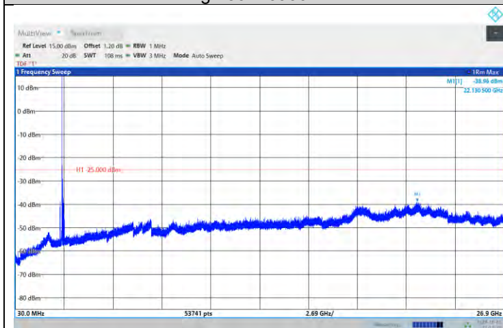
Band41-15MHz-QPSK-39725-1RB#0- Range:30~26900MHz
