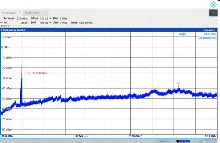
Band41-5MHz-64QAM-40620-1RB#0-Range:30~26900MHz
