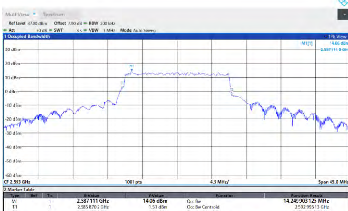
Band41-15MHz-64QAM-39725-75RB#0
