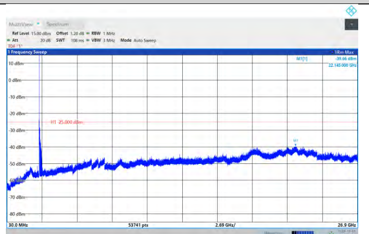
Band41-15MHz-16QAM-41515-1RB#0-Range:30~26900MHz
