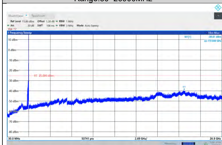
Band41-20MHz-QPSK-40620-1RB#0- Range:30~26900MHz
