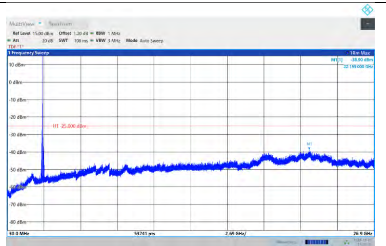
Band41-10MHz-QPSK-39700-1RB#0-Range:30~26900MHz
