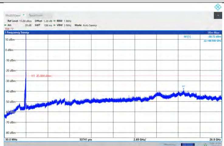
Band41-20MHz-16QAM-40620-1RB#0-Range:30~26900MHz
