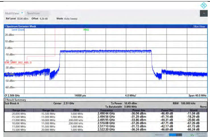
Band41-20MHz-QPSK-41490-100RB#0
