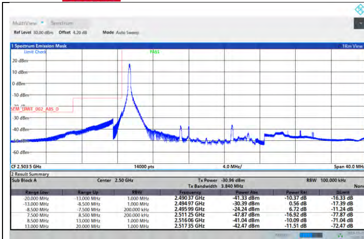
Band41-15MHz-QPSK-41515-1RB#74
