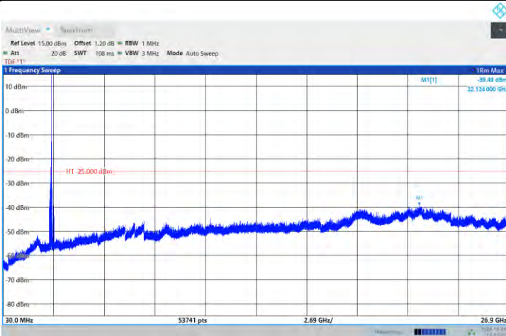
Band41-5MHz-64QAM-39675-1RB#0- Range:30~26900MHz
