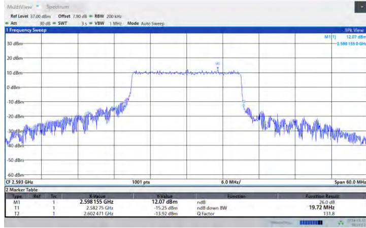
Band41-20MHz-64QAM-40620-100RB#0
