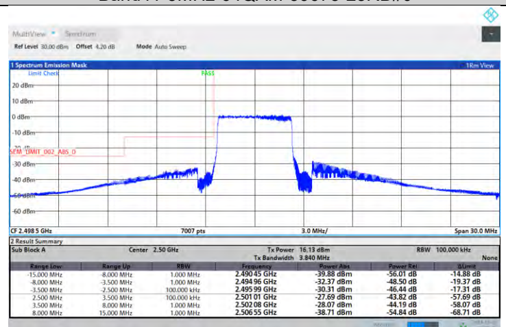
Band41-5MHz-64QAM-41565-25RB#0
