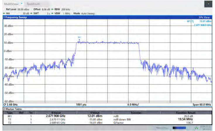
Band41-20MHz-64QAM-41490-100RB#0
