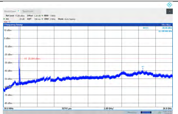
Band41-10MHz-QPSK-41540-1RB#0-Range:30~26900MHz
