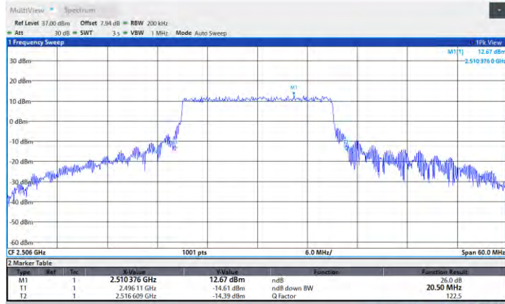
Band41-20MHz-16QAM-41490-100RB#0
