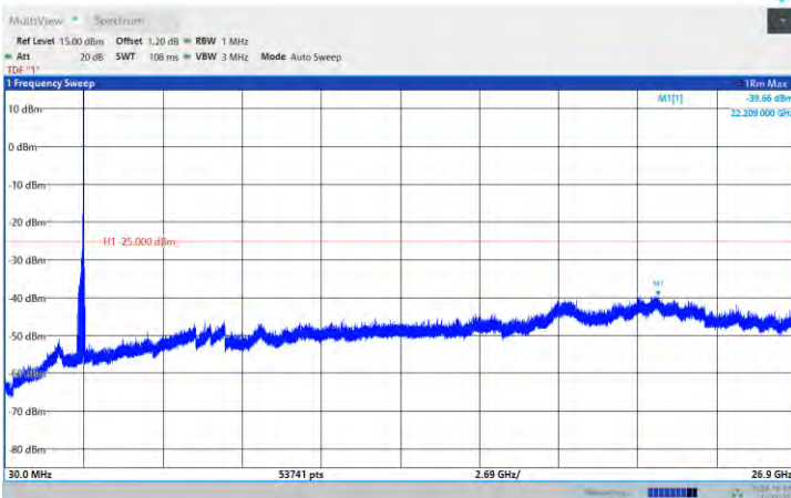
Band41-5MHz-16QAM-40620-1RB#0- Range:30~26900MHz
