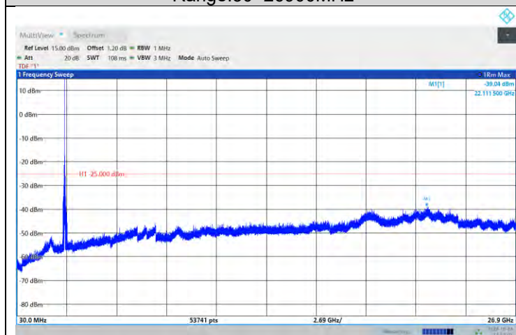
Band41-20MHz-16QAM-39750-1RB#0- Range:30~26900MHz
