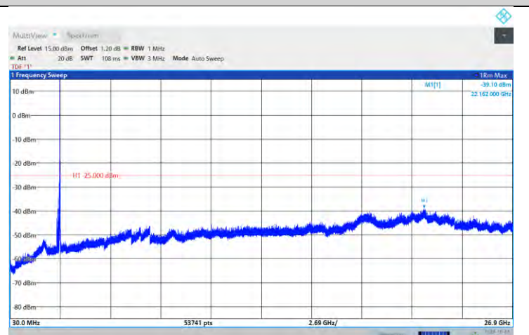
Band41-15MHz-64QAM-40620-1RB#0-Range:30~26900MHz
