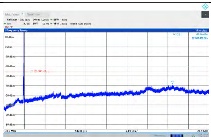
Band41-20MHz-QPSK-39750-1RB#0-Range:30~26900MHz
