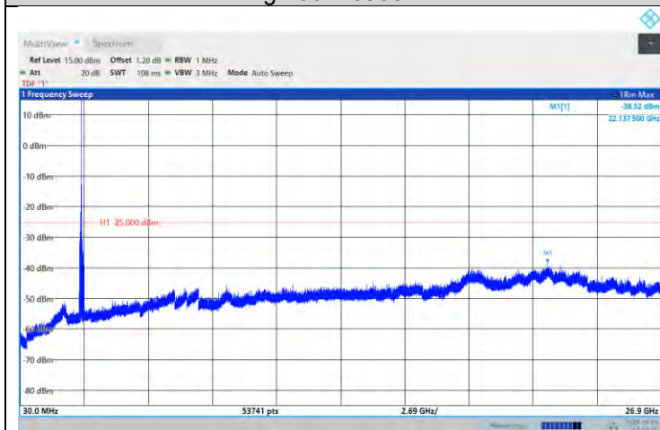
Band41-10MHz-16QAM-39700-1RB#0- Range:30~26900MHz
