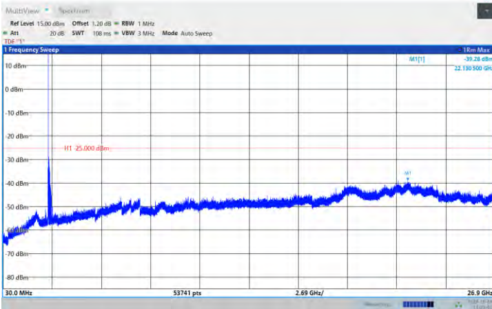
Band41-5MHz-QPSK-41565-1RB#0-Range:30~26900MHz
