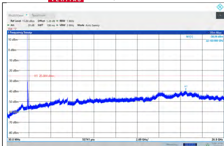
Band41-15MHz-64QAM-41515-1RB#0- Range:30~26900MHz
