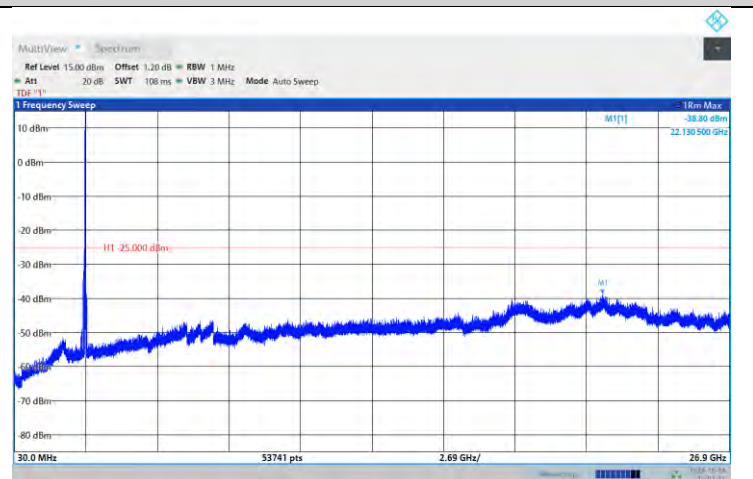
Band41-10MHz-16QAM-40620-1RB#0-Range:30~26900MHz
