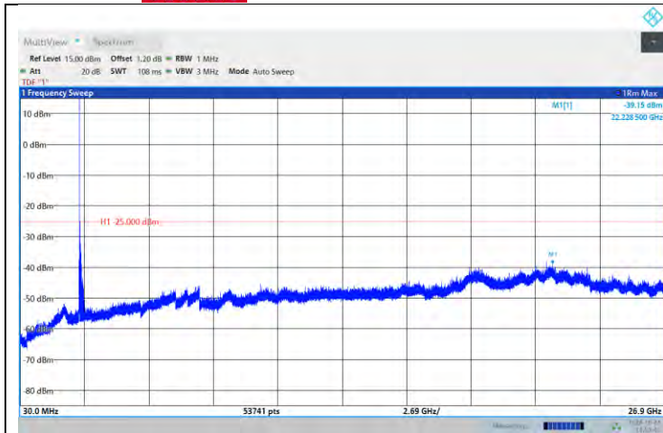
Band41-5MHz-64QAM-41565-1RB#0- Range:30~26900MHz
