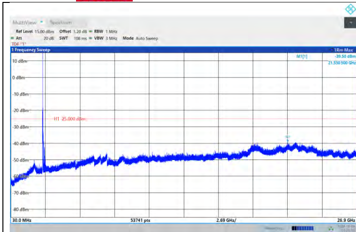
Band41-15MHz-QPSK-41515-1RB#0- Range:30~26900MHz
