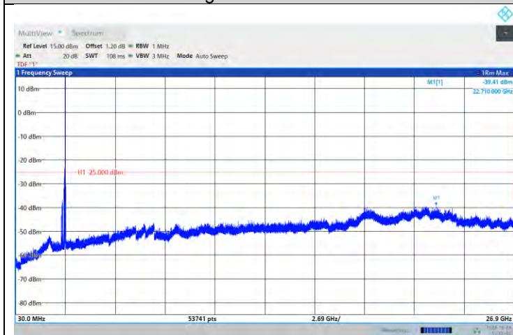
Band41-10MHz-QPSK-40620-1RB#0- Range:30~26900MHz
