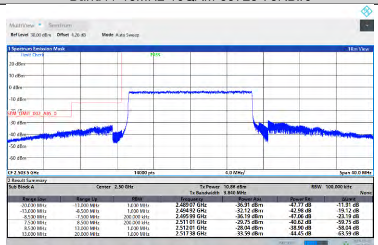
Band41-15MHz-16QAM-41515-75RB#0
