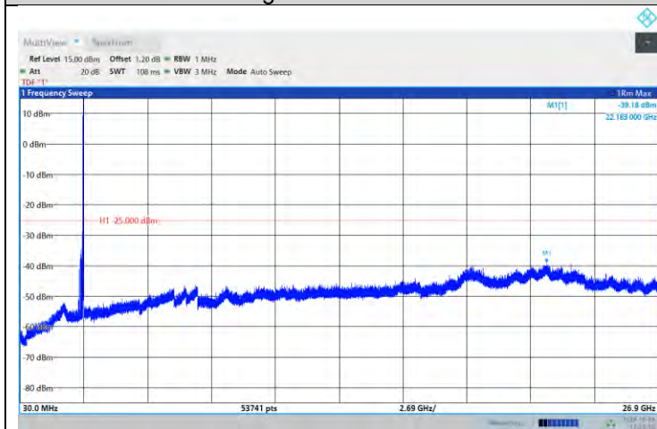
Band41-10MHz-64QAM-40620-1RB#0- Range:30~26900MHz
