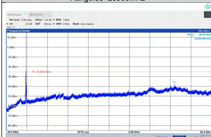
Band41-15MHz-64QAM-39725-1RB#0- Range:30~26900MHz
