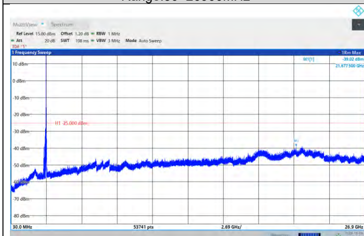
Band41-15MHz-16QAM-40620-1RB#0- Range:30~26900MHz
