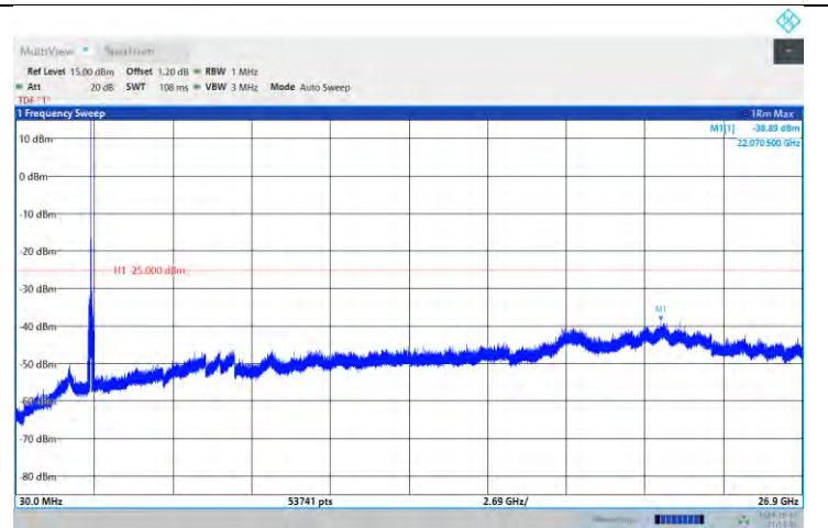
Band41-15MHz-16QAM-39725-1RB#0-Range:30~26900MHz
