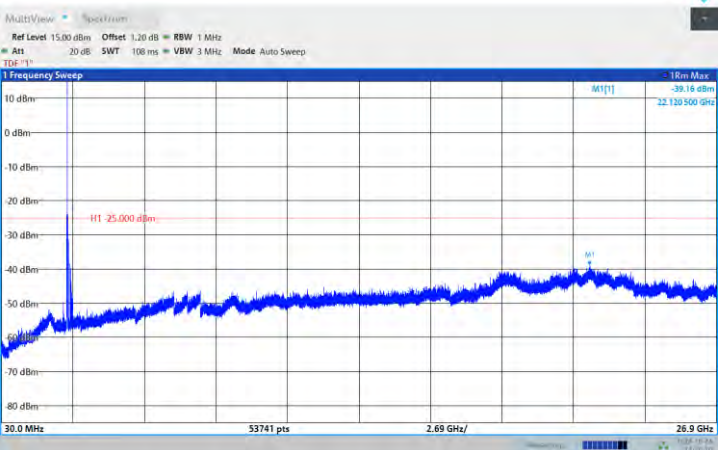
Band41-5MHz-16QAM-41565-1RB#0-Range:30~26900MHz
