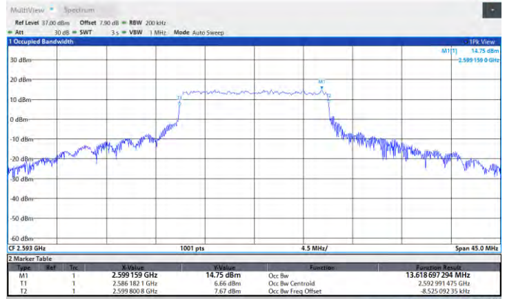
Band41-15MHz-16QAM-39725-75RB#0
