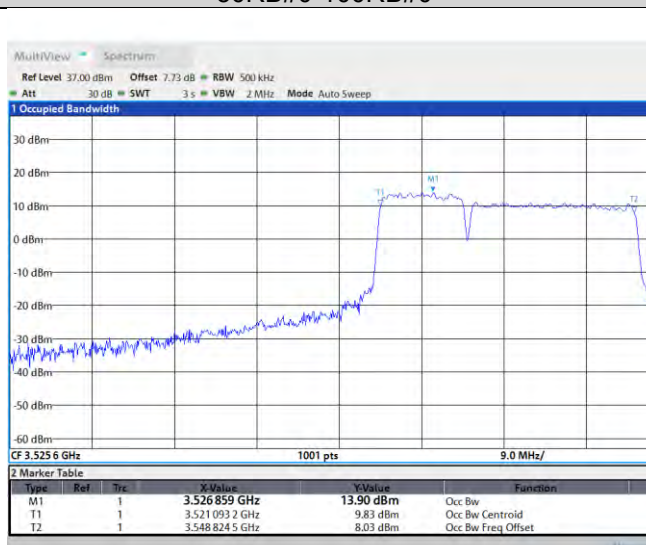
42-42-10MHz-20MHz-64QAM-64QAM-42496-42640- 50RB#0-100RB#0
