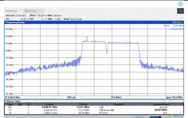
41-41-15MHz-20MHz-64QAM-64QAM-40523-40694-75RB#0-100RB#0
