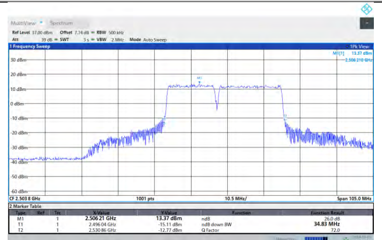
41-41-15MHz-20MHz-16QAM-16QAM-41319-41490-75RB#0-100RB#0
