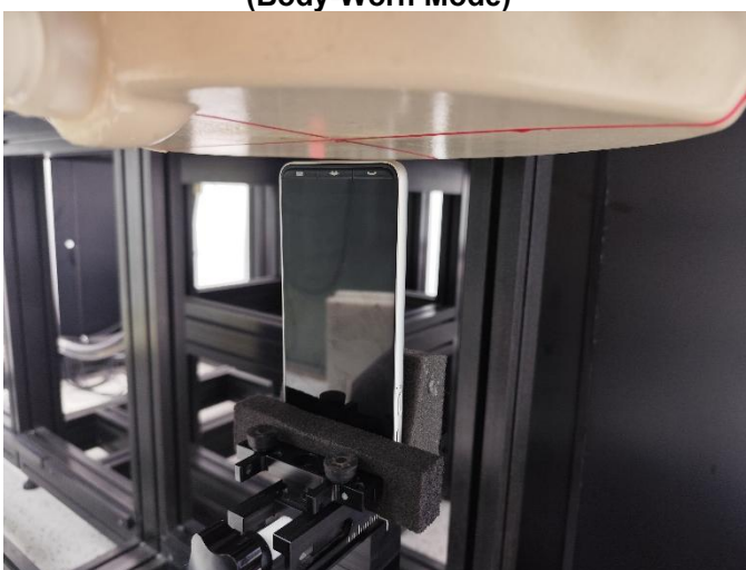
Bottom Side of EUT with 1 cm Gap (Body-Worn Mode)
