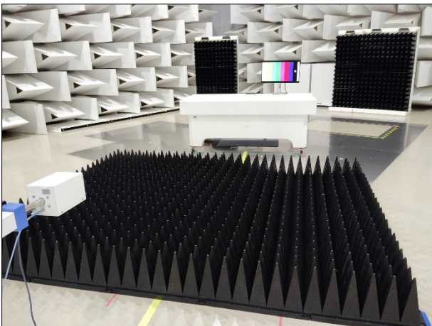
18 GHz-21 GHz
