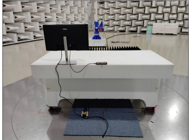
18 GHz-21 GHz
