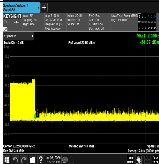
11AX160MIMO-Ant5-6025-High-6098.1014-OFF-PASS
