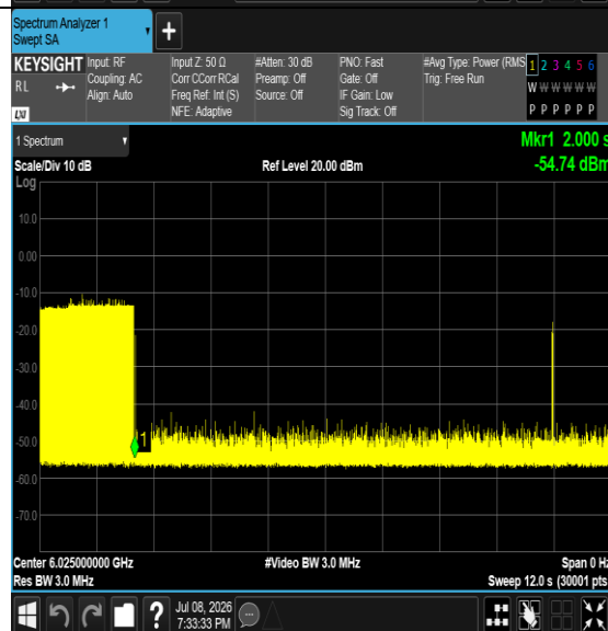
11AX160MIMO-Ant5-6025-High-6098.1014-Minimal
