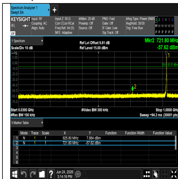
Halow-4M-Ant2-924.5~Reference-PASS
