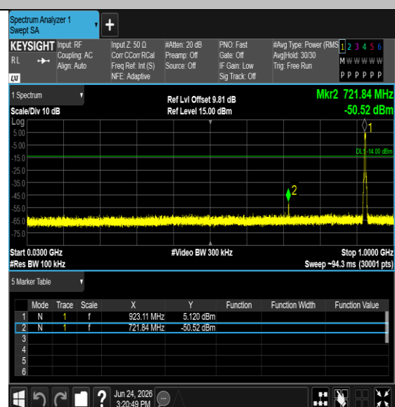
Halow-4M-Ant2-925.5~Reference-PASS
