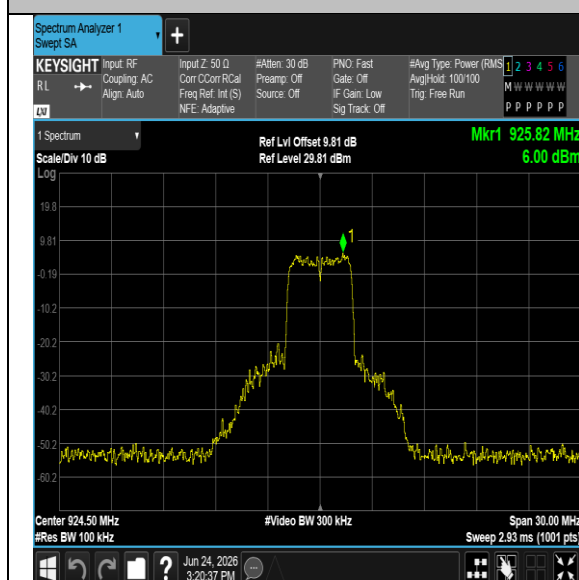
Halow-4M-Ant2-924.5~10000~10000-PASS
