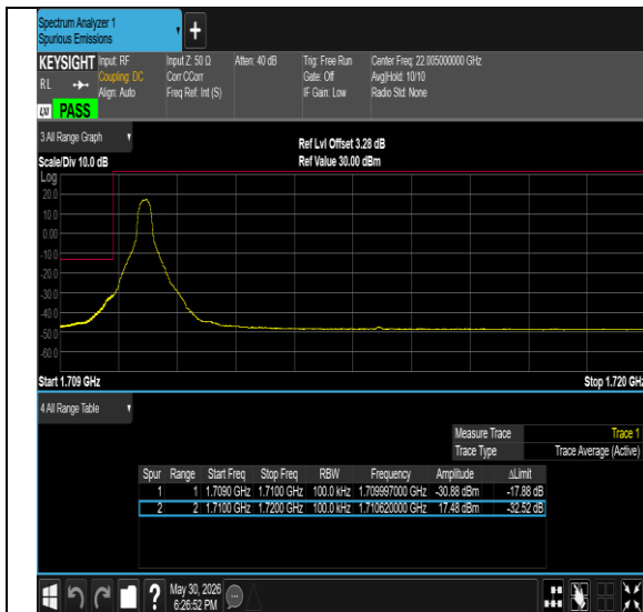
Band4-10MHz-64QAM-20350-1RB#49-PASS
