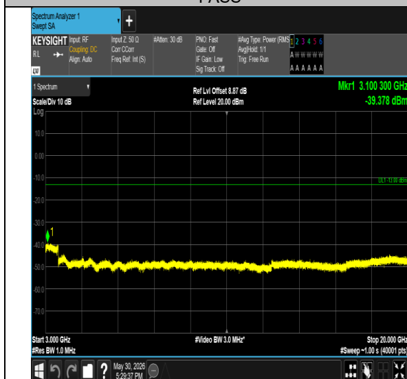
Band4-1.4MHz-QPSK-20393-1RB#0-3000~20000-PASS
