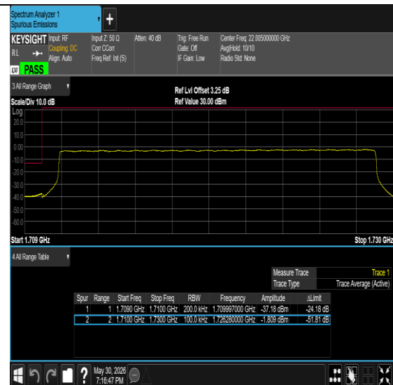
Band4-20MHz-64QAM-20300-100RB#0-PASS
