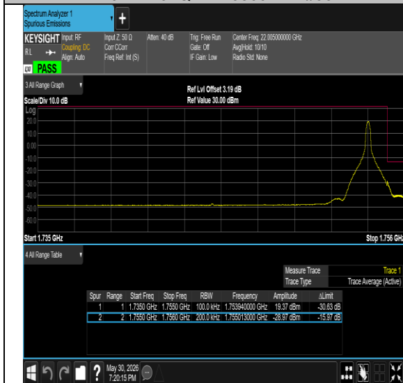
Band4-20MHz-16QAM-20050-1RB#0-PASS
