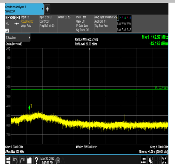
Band4-3MHz-QPSK-19965-1RB#0-30~1000-PASS
