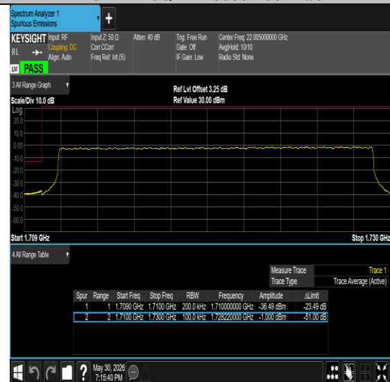
Band4-20MHz-16QAM-20300-100RB#0-PASS
