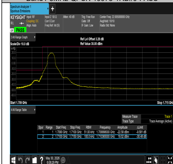
Band4-5MHz-QPSK-20375-1RB#24-PASS
