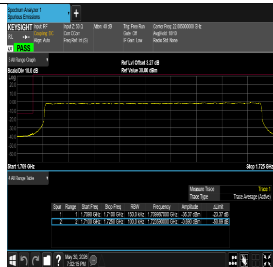
Band4-15MHz-64QAM-20325-75RB#0-PASS
