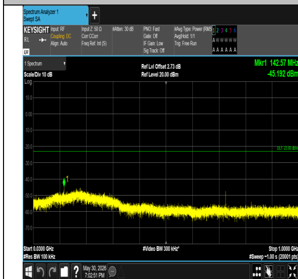
Band4-20MHz-QPSK-20050-1RB#0-30~1000-PASS
