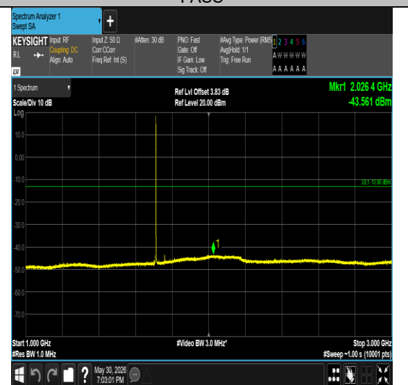
Band4-20MHz-QPSK-20050-1RB#0-1000~3000-PASS
