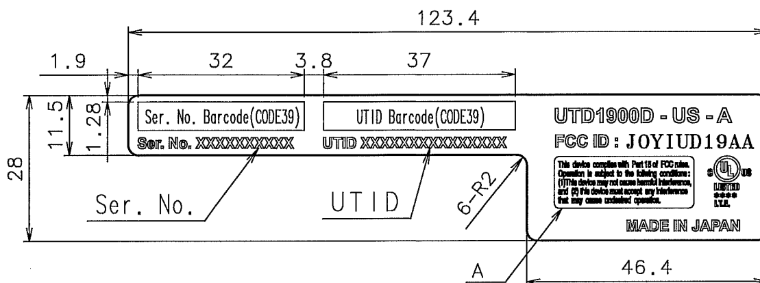
SCALE 1/1 Detail of SERIAL NO.PLATE
