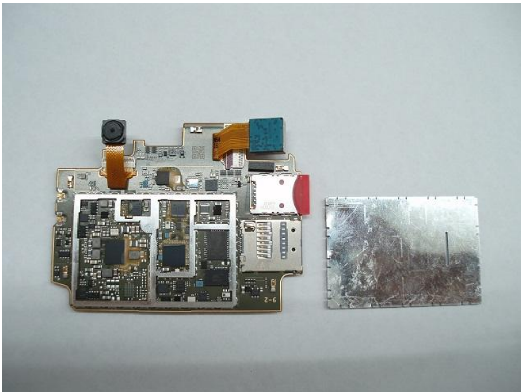
Main PCB Back View without Shield
