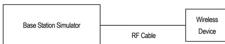
Figure 10.3 Power Measurement Setup
