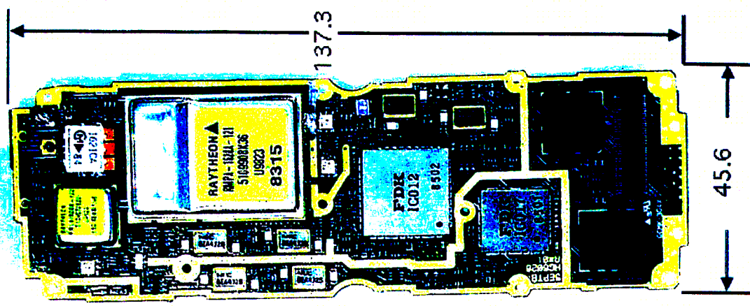
TOP OF SS-66K/SD-66K RF BOARD
