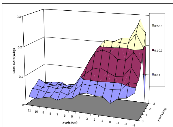
Figure 3. Antenna In
