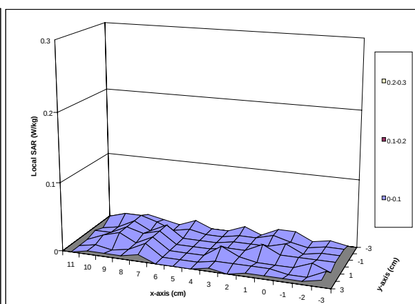
Figure 4. Antenna Out
