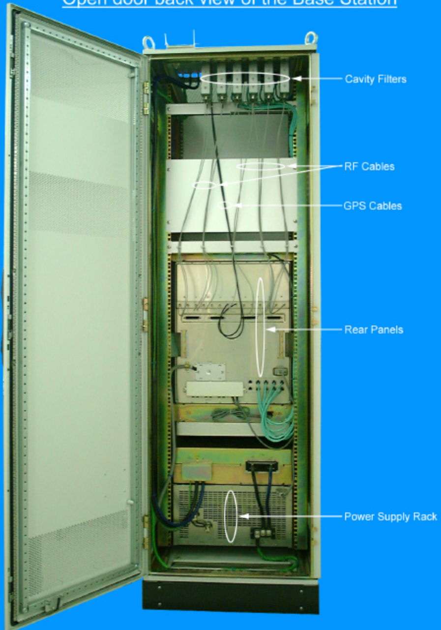
Open door back view of the Base Station
