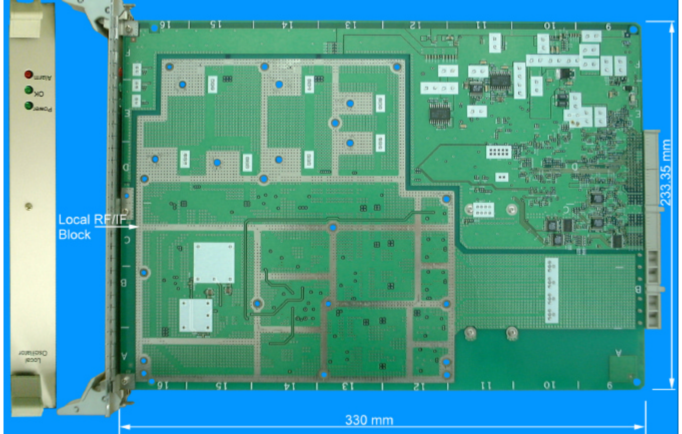
Bottom side of the Local Oscillator Module Board
