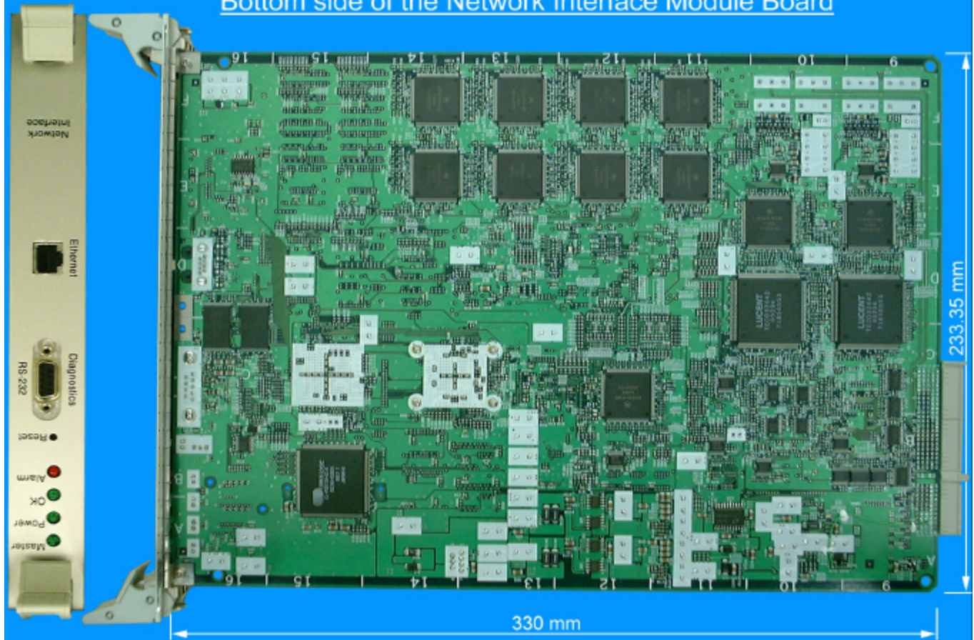
Bottom side of the Network Interface Module Board
