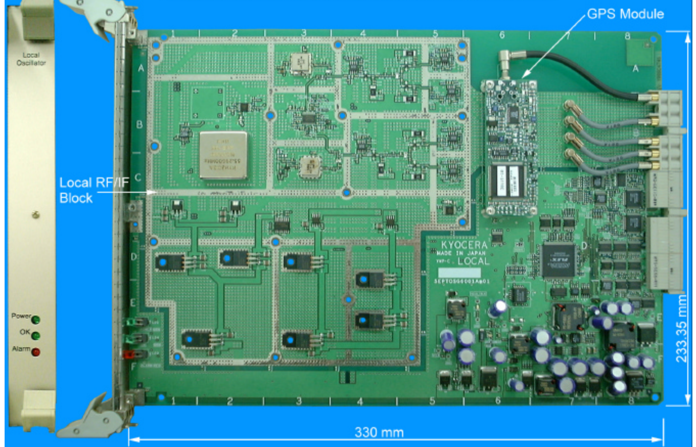
Top side of the Local Oscillator Module Board
