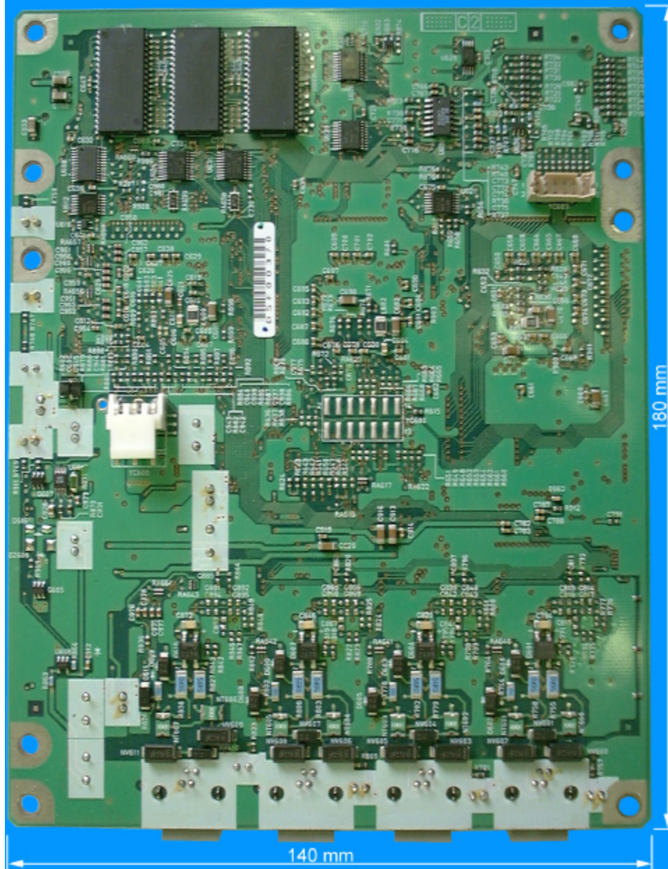
Bottom side of the FLSU Digital Board
