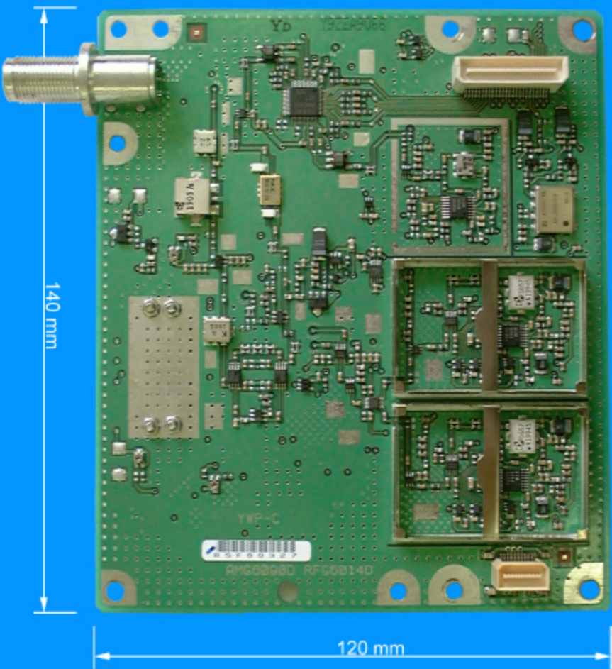
Bottom side of the FLSU RF Board
